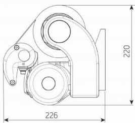
Wall mounting
